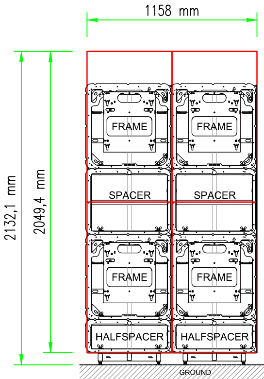
adjustable foot \pm 15 mm front view
