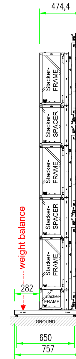
side view 02 base position front
