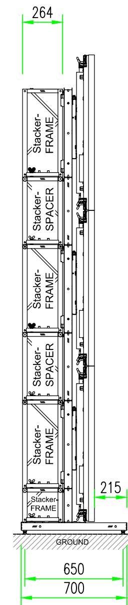
side view 01 base position middle
